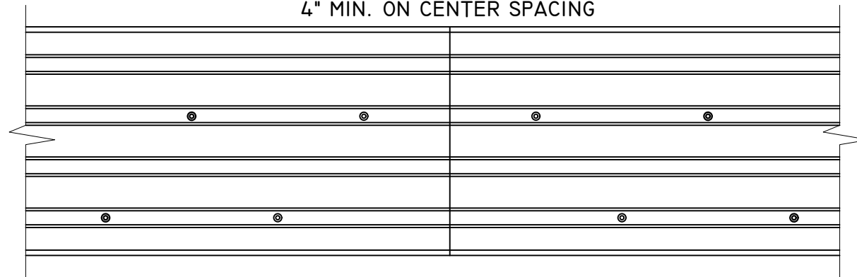
4-0 MAX. PANEL TYPICAL PATTERN AT SPLICE SEE TABLE 1, SHEET 2: ANCHORS L & M 4" MIN. ON CENTER SPACING
