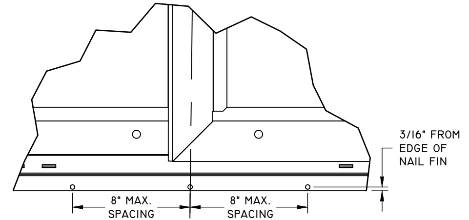
DETAIL B
