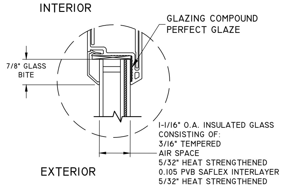
GLAZING DETAIL 2
